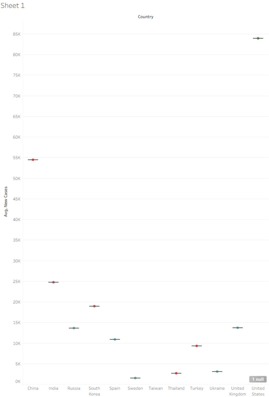
Chart 1: Boxplot (Distribution)
